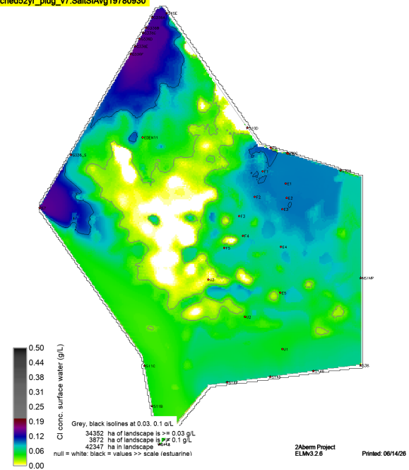
sched52yr_plug_v7.SaltSAvg19780930
