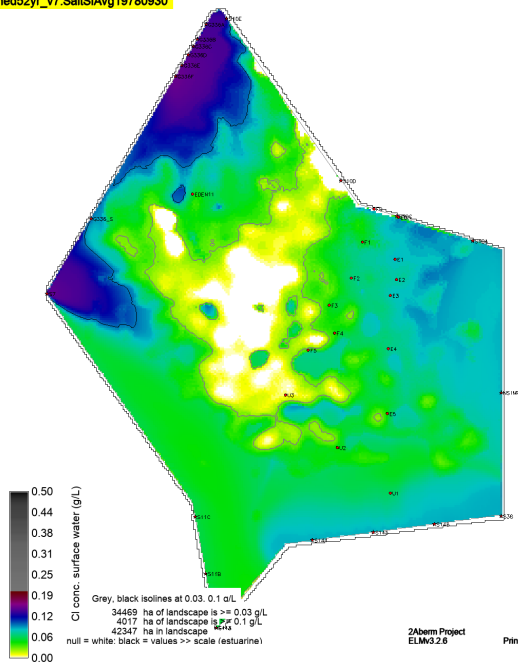
sched52yr_v7.SaltSAvg19780930
