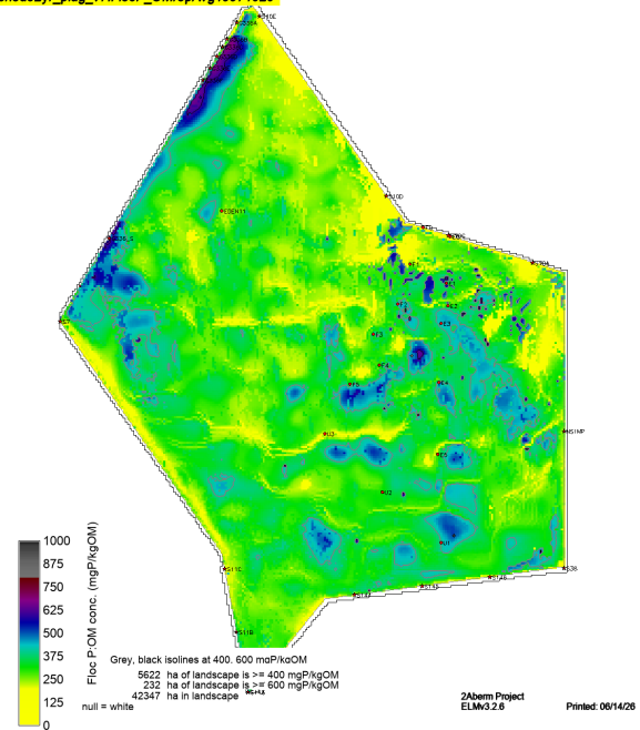
sched52yr_plug_v7.FlocP_OMrepAvg19971020
