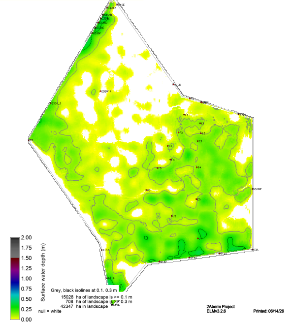
sched52yr_plug_v7.HydRelDepPosNegAvg_POSmean
