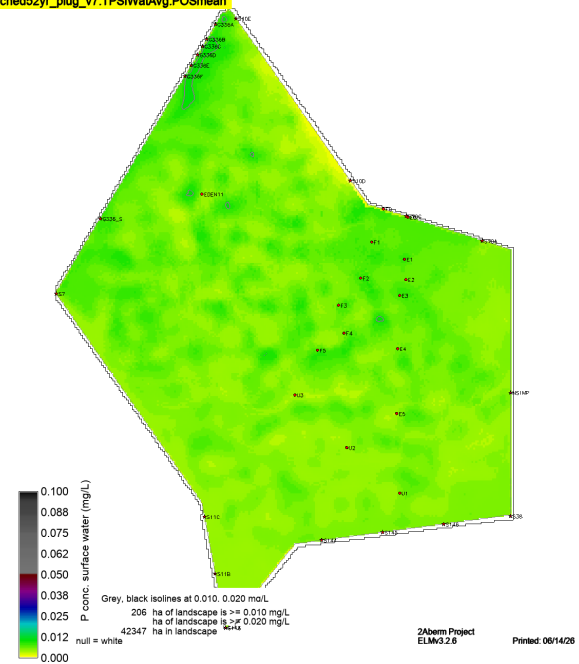
sched52yr_plug_v7.TPSWatAvg.POSmean
