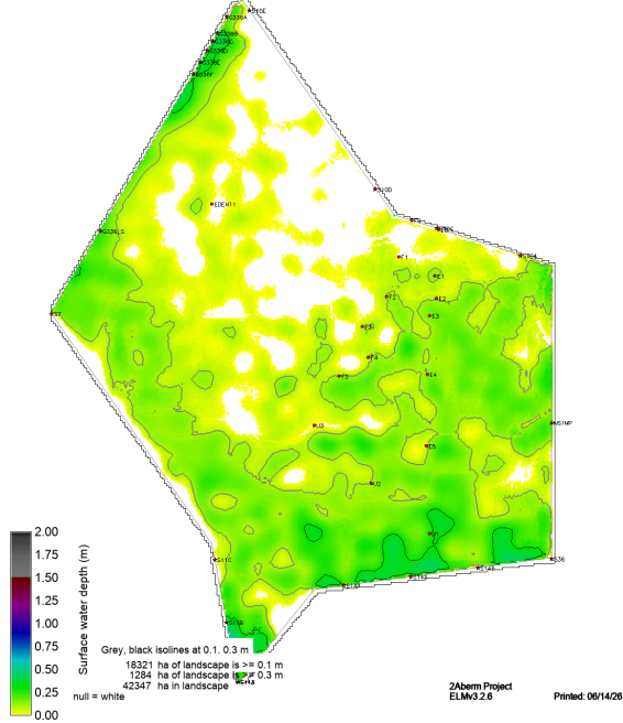
sched52yr_v7.HydRelDepPosNegAvg_POSmean
