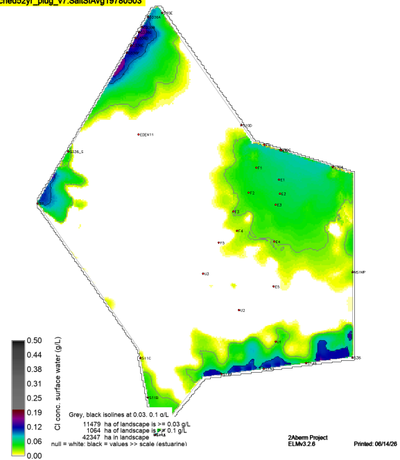
sched52yr_plug_v7.SaltSAvg19780503
