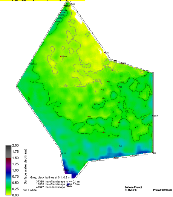
sched52yr_plug_v7.HydRelDepPosNegAvg19971020
