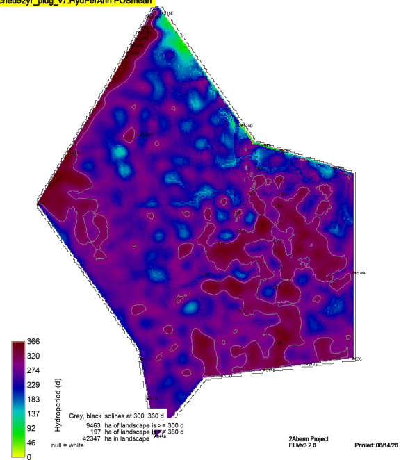
sched52yr_plug_v7.HydPerAnn.POSmean
