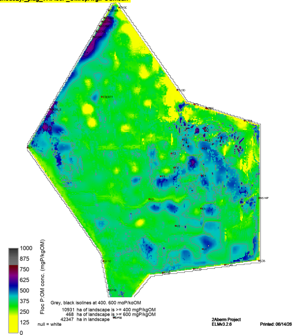
sched52yr_plug_v7.FlocP_OMrepAvg.POSmean
