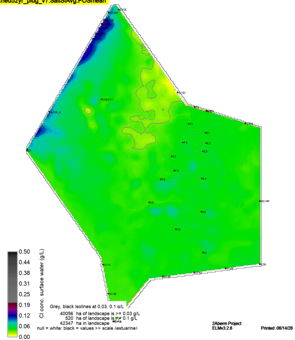
sched52yr_plug_v7.SaltSAvg.POSmean
