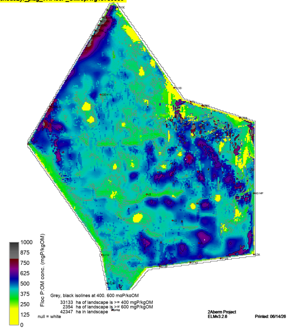
sched52yr_plug_v7.FlocP_OMrepAvg19780930
