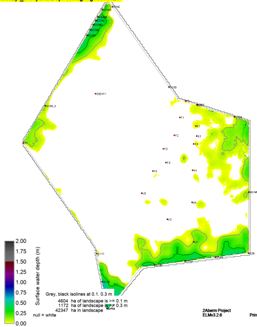
sched52yr_v7.HydRelDepPosNegAvg19970423
