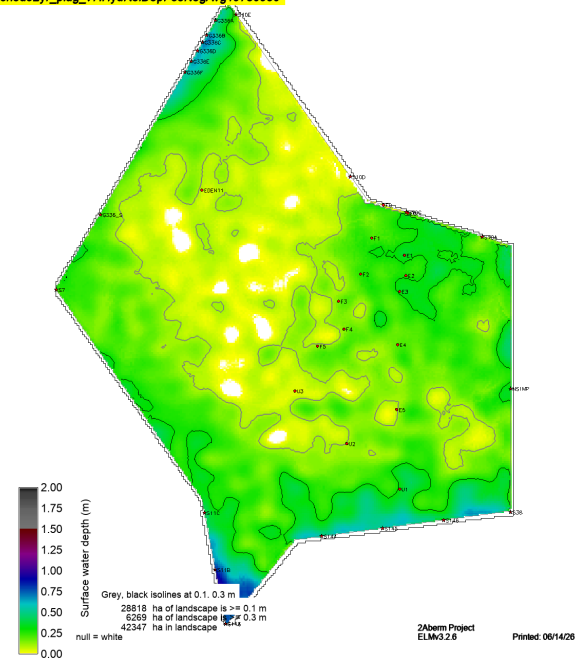
sched52yr_plug_v7.HydRelDepPosNegAvg19780930
