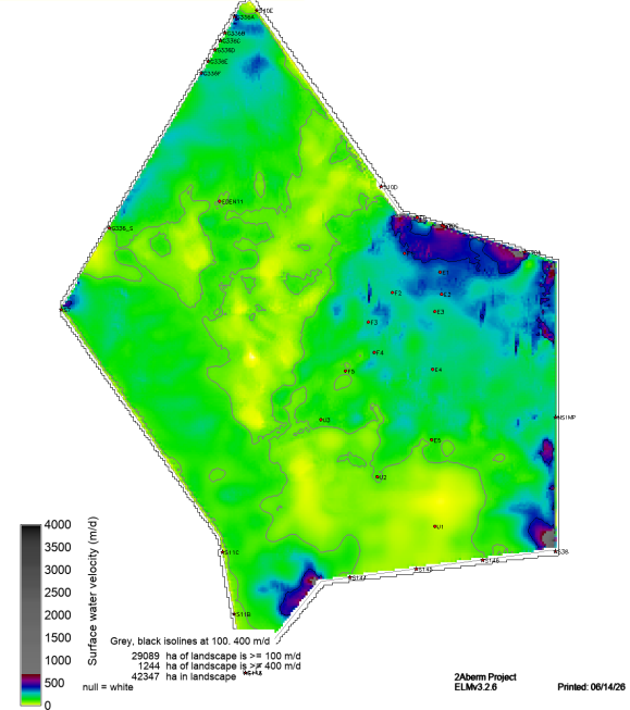
sched52yr_plug_v7_SF_WT_VEL_magAvg19780930
