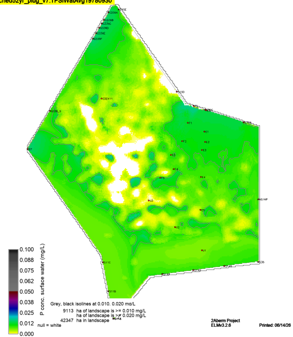
sched52yr_plug_v7.TPSWtaAvg19780930
