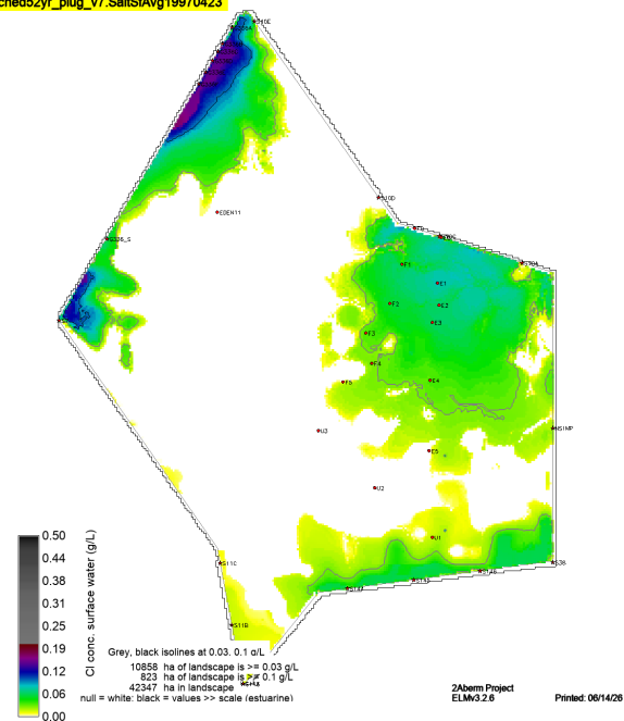
sched52yr_plug_v7.SaltSAvg19970423
