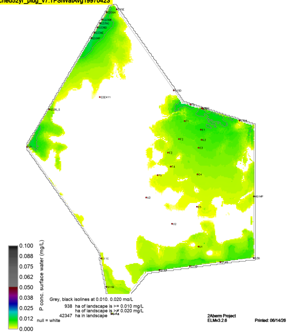
sched52yr_plug_v7.TPSWtAvg19970423
