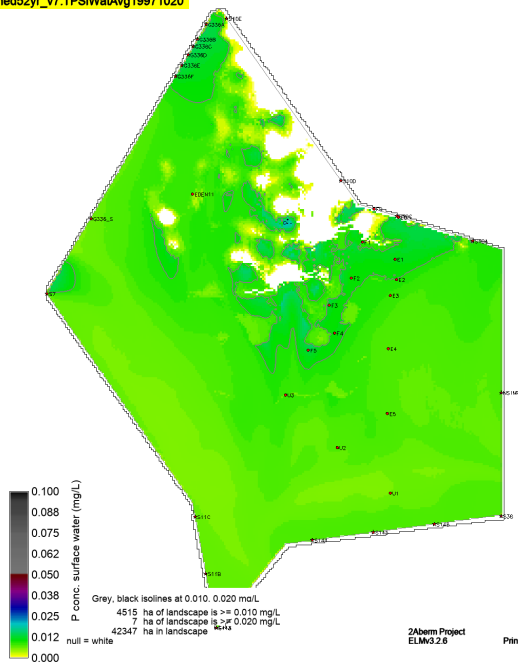
sched52yr_v7.TPSWwAvg19971020
