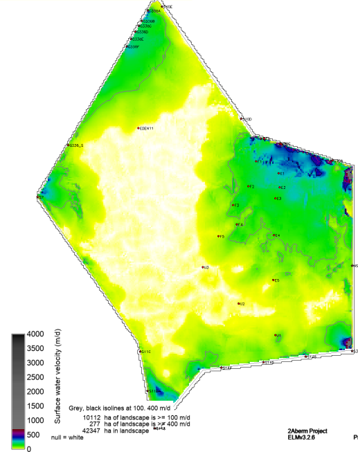
sched52yr_plug_v7_SF_WT_VEL_magAvg19970423
