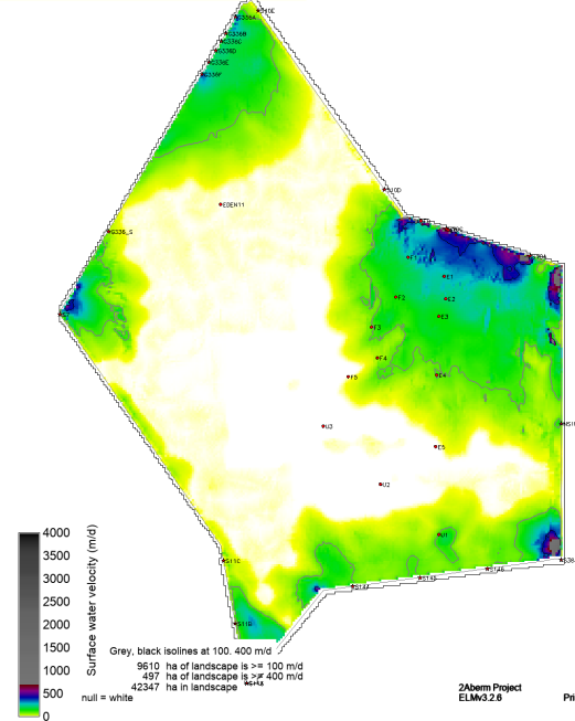
sched52yr_plug_v7_SF_WT_VEL_magAvg19780503
