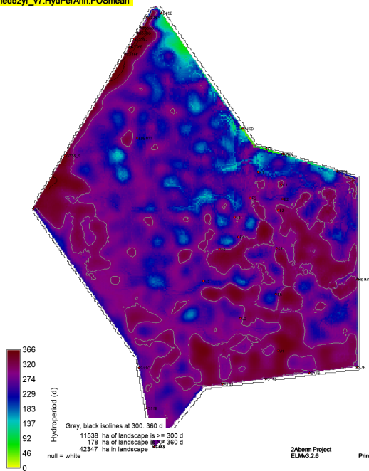
sched52yr_v7.HydPerAnn.POSmean
