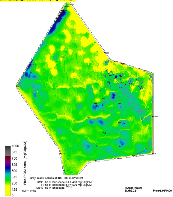
sched52yr_plug_v7.FlocP_OMrepAvg19970423
