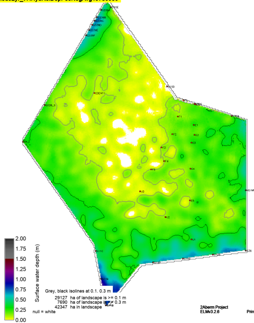
sched52yr_v7.HydRelDepPosNegAvg19780930
