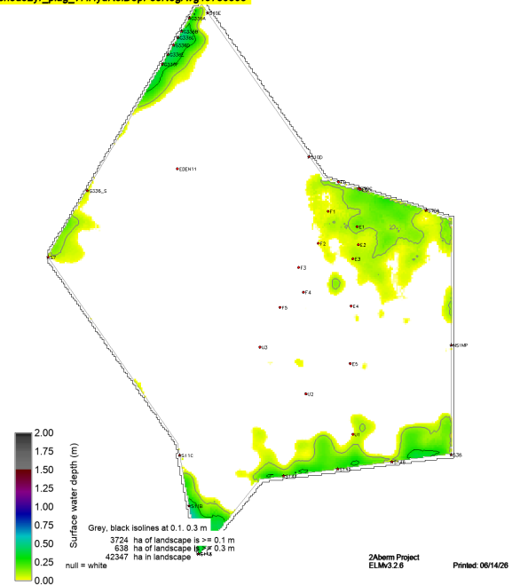
sched52yr_plug_v7.HydRelDepPosNegAvg19780503
