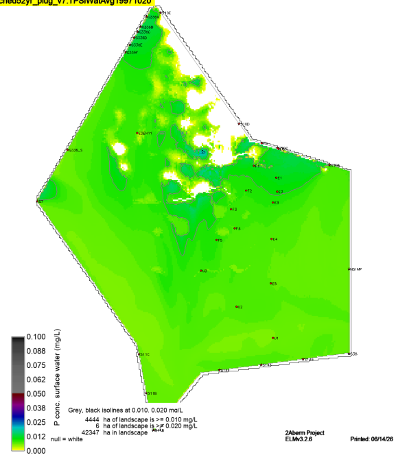
sched52yr_plug_v7.TPSWwAvg19971020
