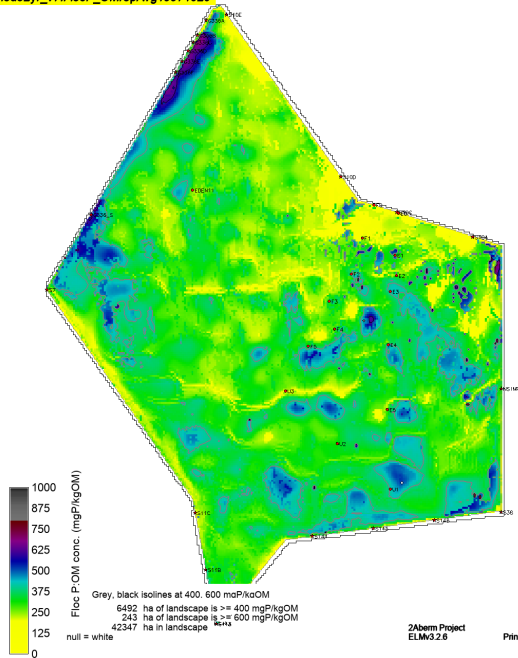
sched52yr_v7.FlocP_OMrepAvg19971020
