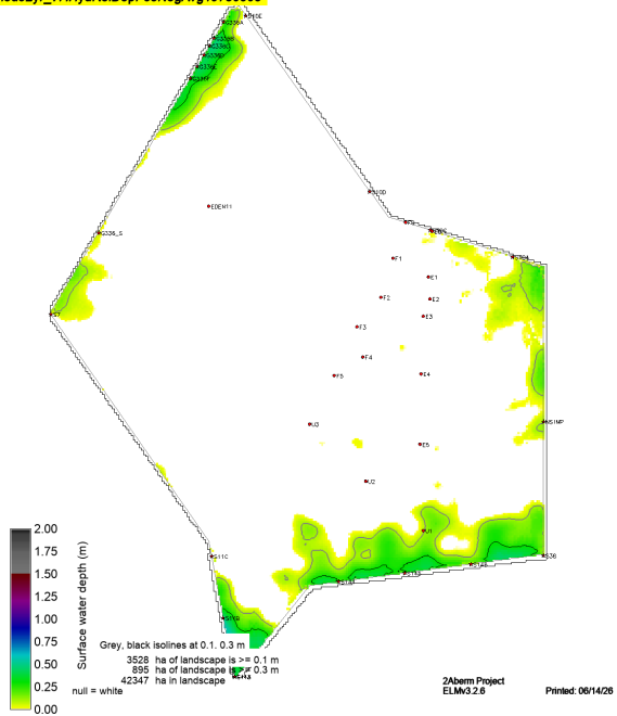
sched52yr_v7.HydRelDepPosNegAvg19780503
