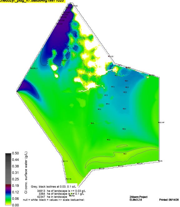
sched52yr_plug_v7.SaltSAvg19971020
