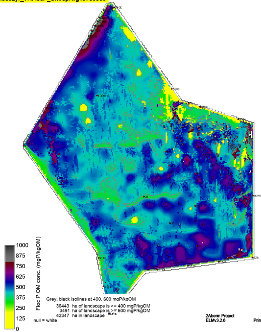
sched52yr_v7.FlocP_OMrepAvg19780930
