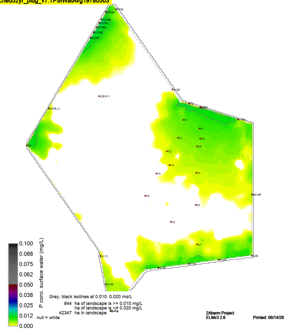
sched52yr_plug_v7.TPSWwAvg19780503
