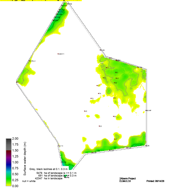
sched52yr_plug_v7.HydRelDepPosNegAvg19970423
