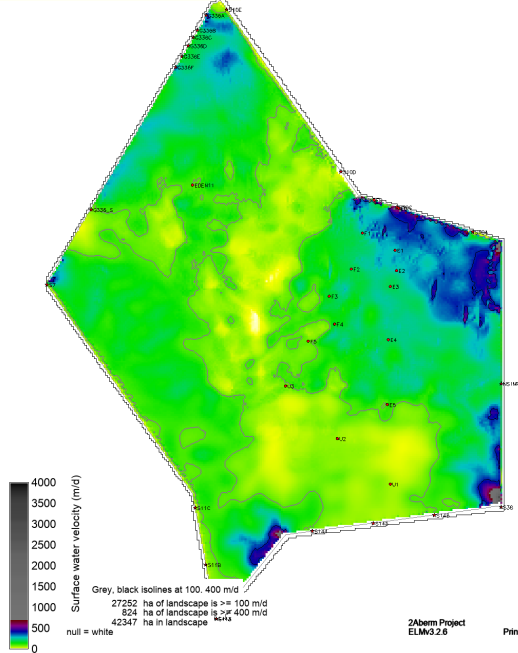
sched52yr_v7_SF_WT_VEL_magAvg19780930
