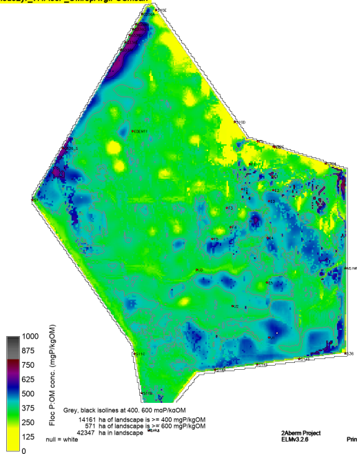
sched52yr_v7.FlocP_OMrepAvg.POSmean
