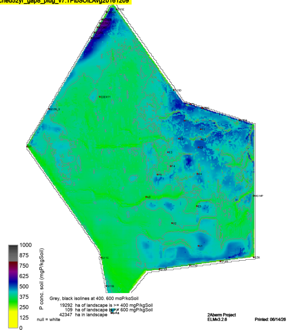
sched52yr_gap8_plug_v7.TPtoSOILAvg20161209
