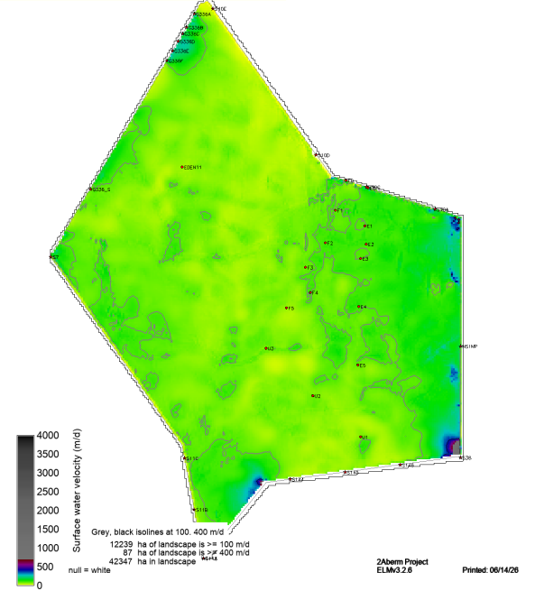
sched52yr_gap8_plug_v7_SF_WT_VEL_magAvg.POSmean
