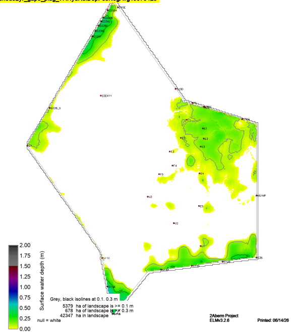
sched52yr_gap8_plug_v7.HydRelDepPosNegAvg19970423
