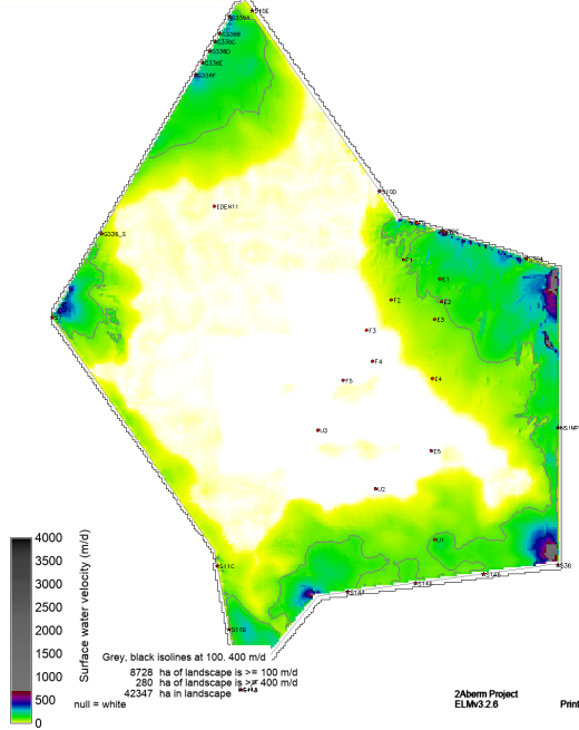
sched52yr_v7_SF_WT_VEL_magAvg19780503
