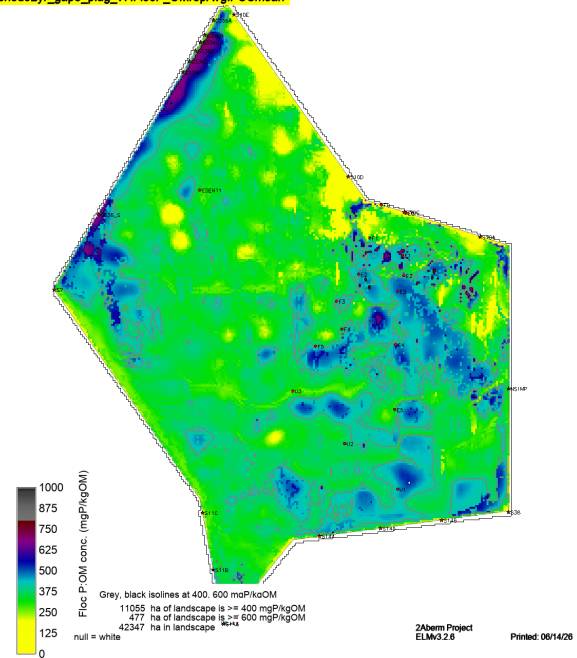
sched52yr_gap8_plug_v7.FlocP_OMrepAvg.POSmean
