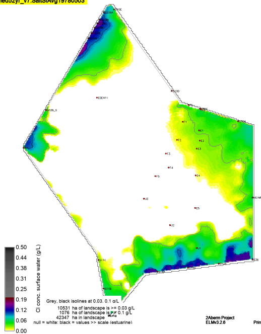
sched52yr_v7.SaltSAvg19780503
