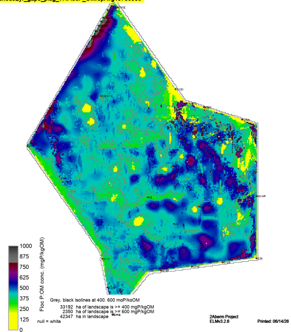
sched52yr_gap8_plug_v7.FlocP_OMrepAvg19780930
