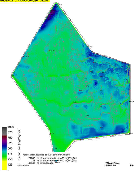
sched52yr_v7.TPtoSOILAvg20161209
