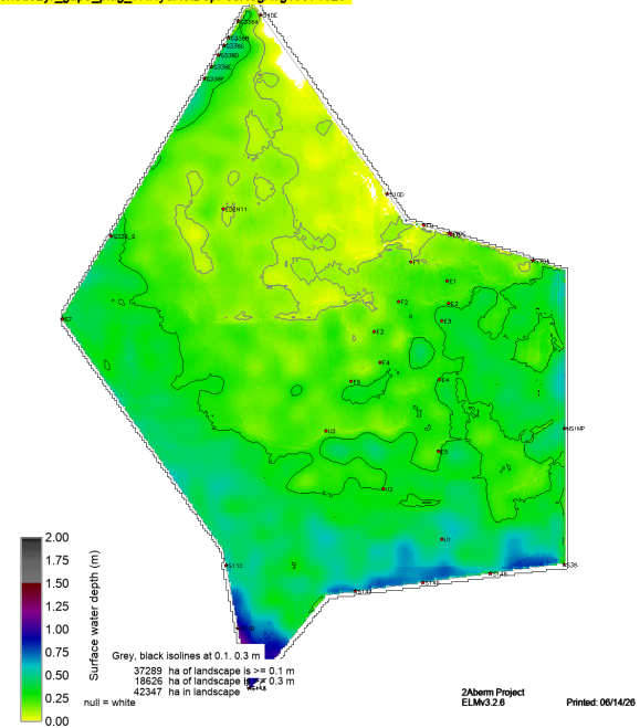
sched52yr_gap8_plug_v7.HydRelDepPosNegAvg19971020
