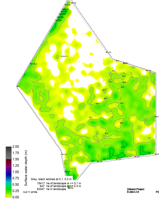
sched52yr_gap8_plug_v7.HydRelDepPosNegAvg.POSmean
