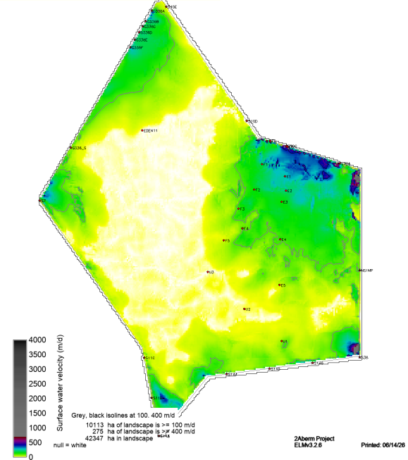
sched52yr_gap8_plug_v7_SF_WT_VEL_magAvg19970423
