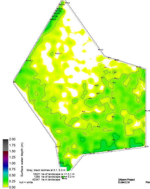
sched52yr_v7.HydRelDepPosNegAvg.POSmean
