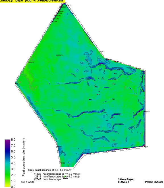
sched52yr_gap8_plug_v7.PeatAccreteRate
