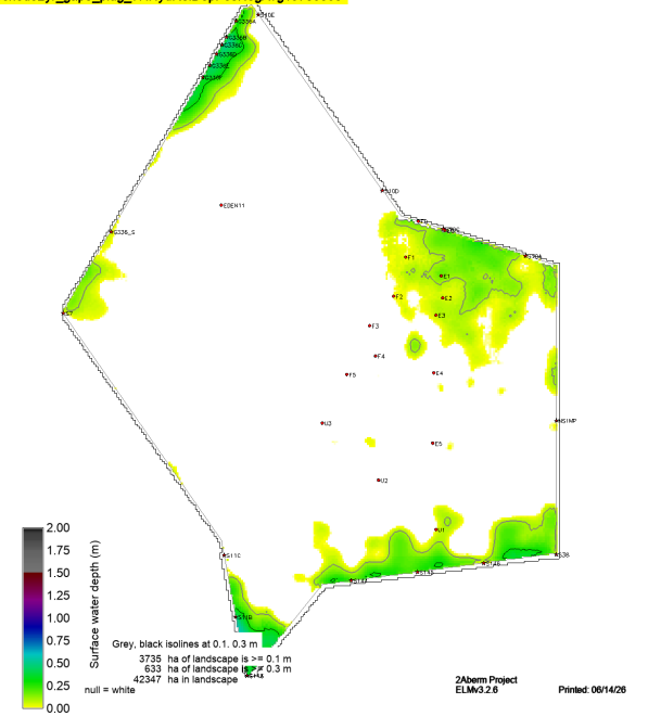
sched52yr_gap8_plug_v7.HydRelDepPosNegAvg19780503
