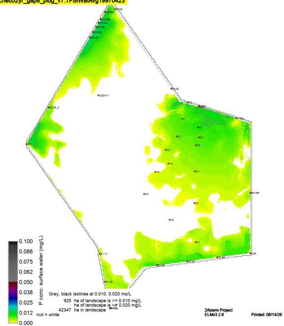
sched52yr_gap8_plug_v7.TPSWatAvg19970423
