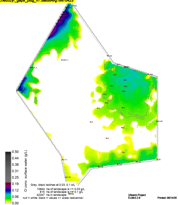
sched52yr_gap8_plug_v7.SaltSAvg19970423
