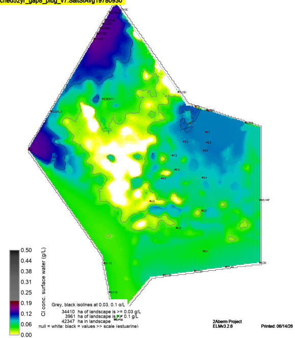
sched52yr_gap8_plug_v7.SaltSAvg19780930
