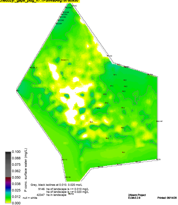
sched52yr_gap8_plug_v7.TPSWatAvg19780930
