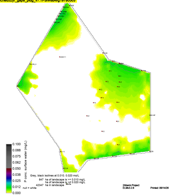
sched52yr_gap8_plug_v7.TPSWatAvg19780503
