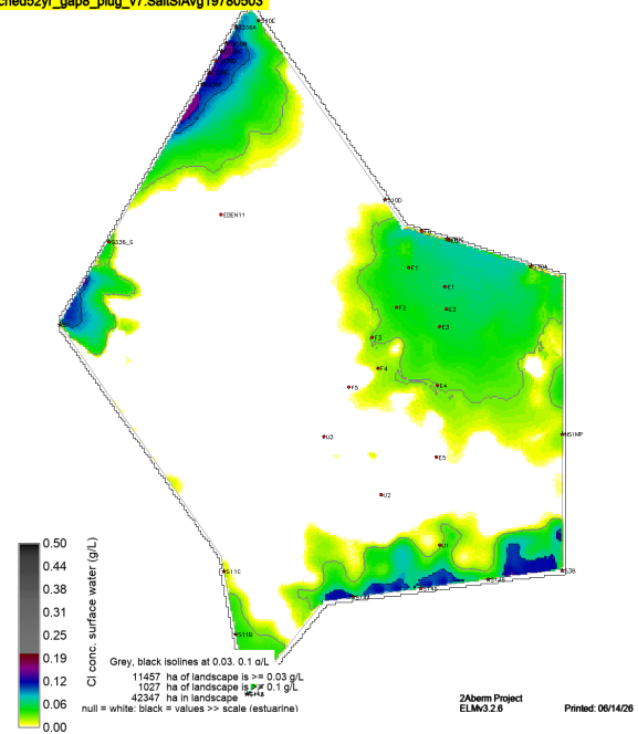
sched52yr_gap8_plug_v7.SaltSAvg19780503
