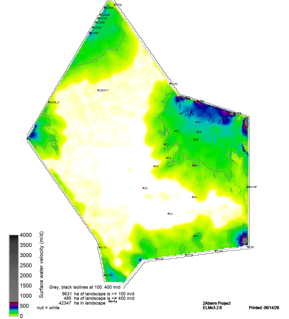
sched52yr_gap8_plug_v7_SF_WT_VEL_magAvg19780503
