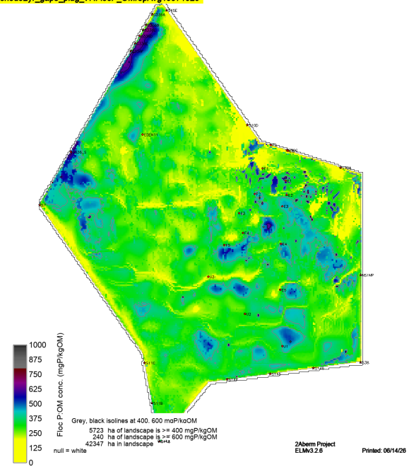
sched52yr_gap8_plug_v7.FlocP_OMrepAvg19971020
