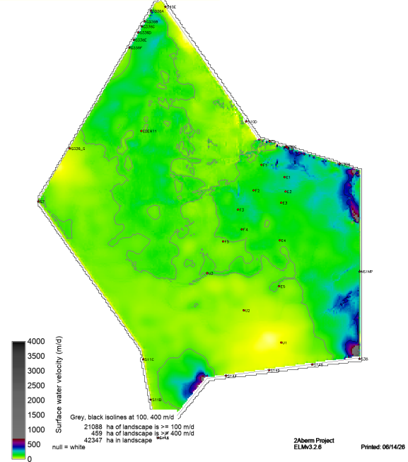
sched52yr_gap8_plug_v7_SF_WT_VEL_magAvg19971020
