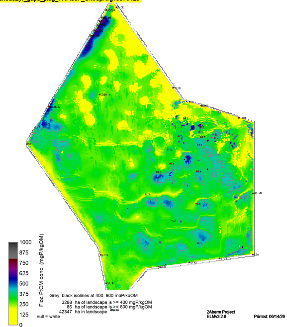
sched52yr_gap8_plug_v7.FlocP_OMrepAvg19970423
