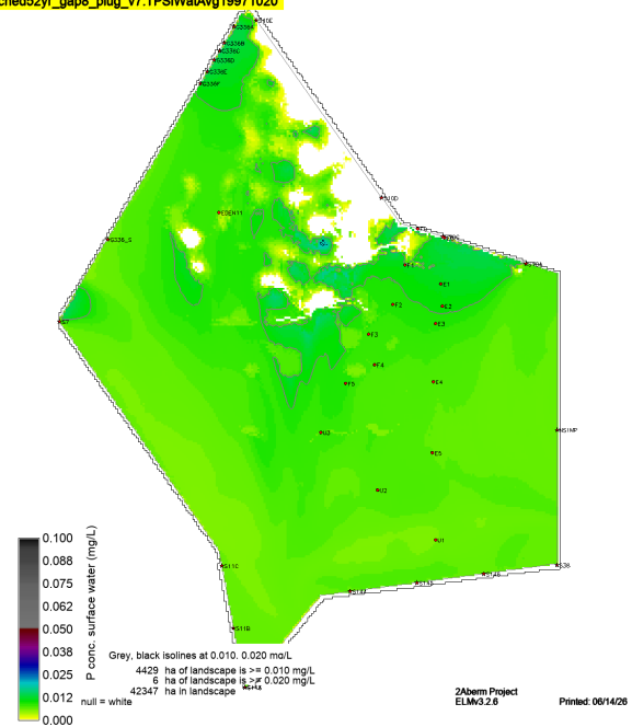
sched52yr_gap8_plug_v7.TPSWatAvg19971020
