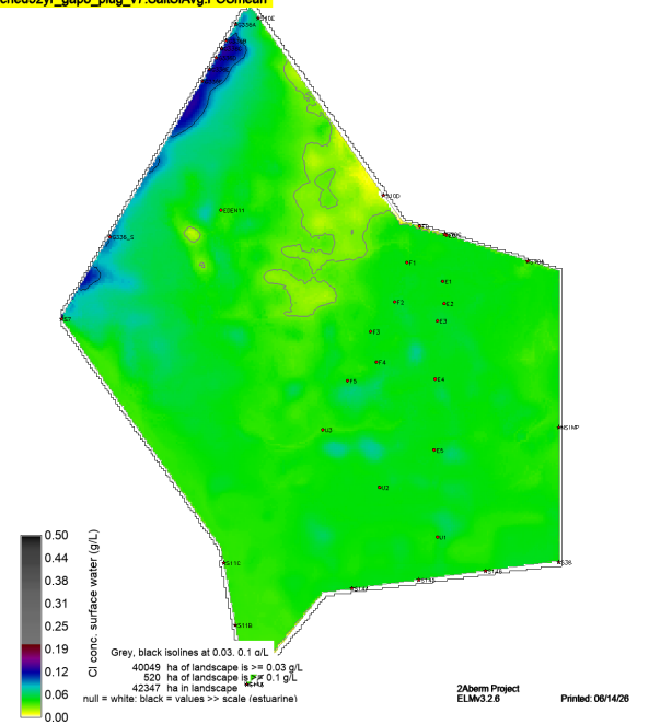
sched52yr_gap8_plug_v7.SaltSAvg.POSmean
