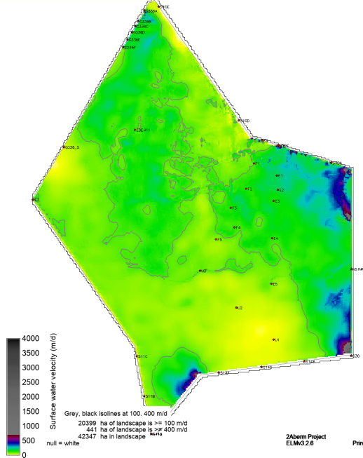
sched52yr_v7_SF_WT_VEL_magAvg19971020
