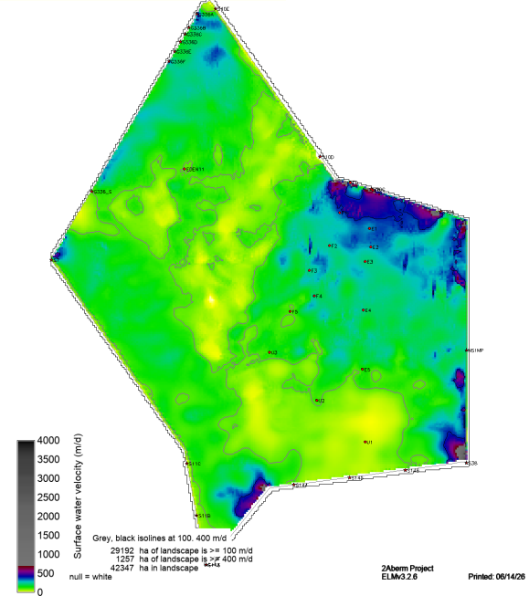
sched52yr_gap8_plug_v7_SF_WT_VEL_magAvg19780930
