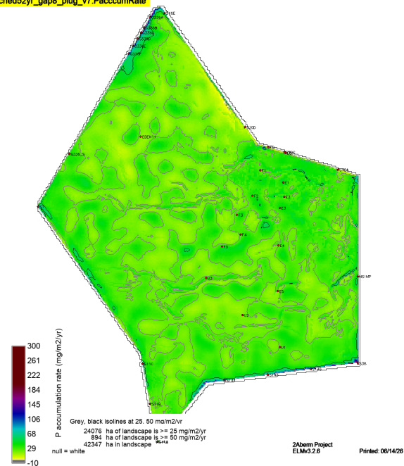
sched52yr_gap8_plug_v7.PaccumRate
