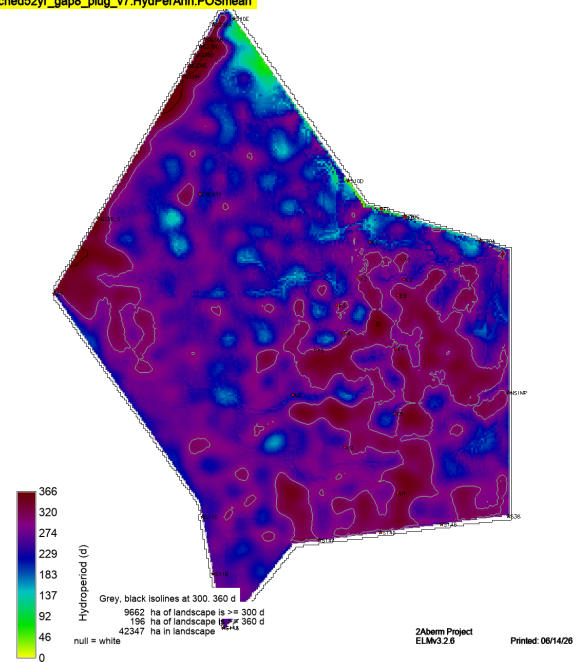
sched52yr_gap8_plug_v7.HydPerAnn.POSmean
