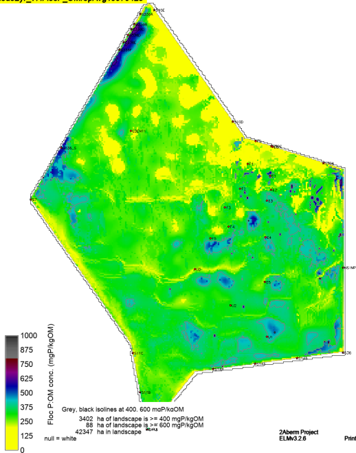
sched52yr_v7.FlocP_OMrepAvg19970423
