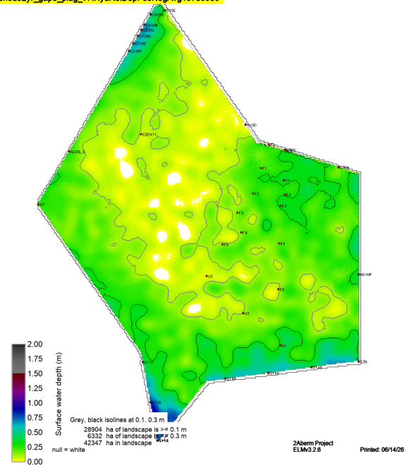
sched52yr_gap8_plug_v7.HydRelDepPosNegAvg19780930
