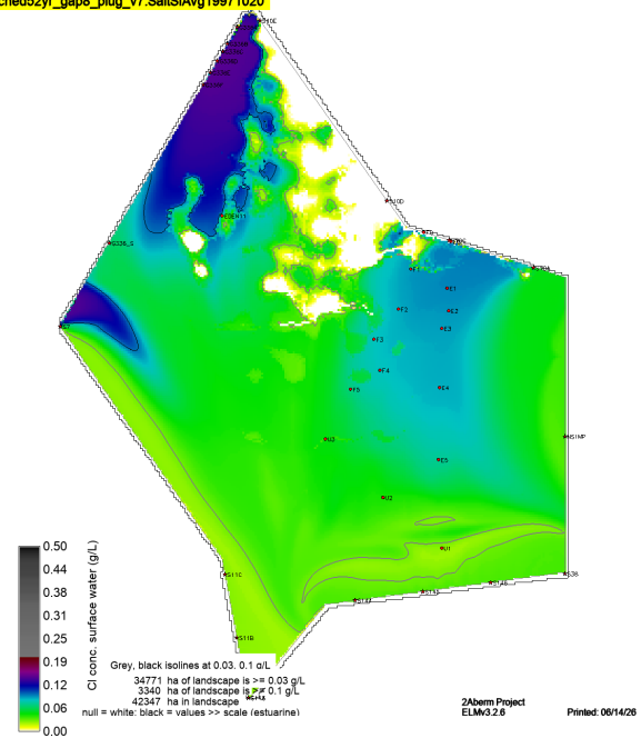
sched52yr_gap8_plug_v7.SaltSAvg19971020
