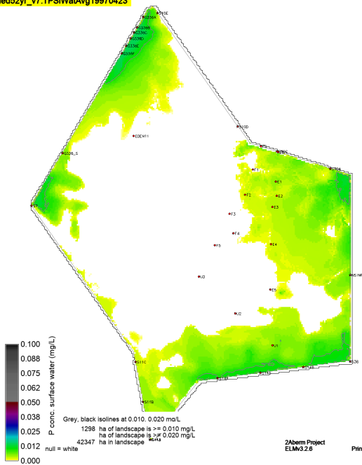
sched52yr_v7.TPSWatAvg19970423
