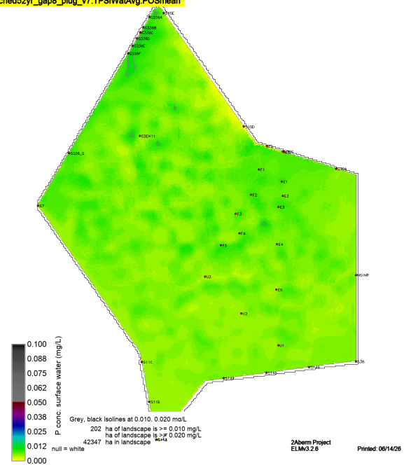
sched52yr_gap8_plug_v7.TPSWatAvg.POSmean
