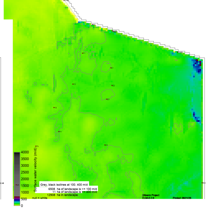
sched52yr_gap8_plug_v7_SF_WT_VEL_magAvg.POSmean
