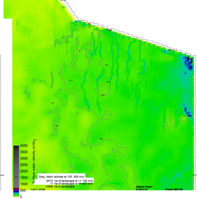
sched52yr_gap8_AMI234_plug_v7_SF_WT_VEL_magAvg.POSmean
