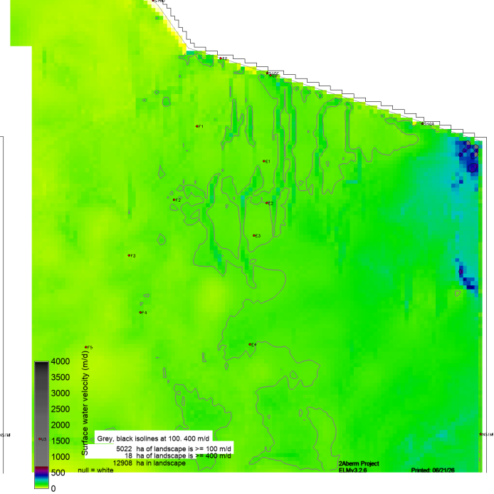
sched52yr_gap8_AMI234_v7_SF_WT_VEL_magAvg.POSmean
